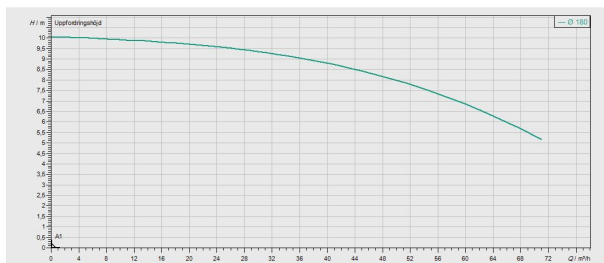
Wilo IPn 80/180-2.2/4
